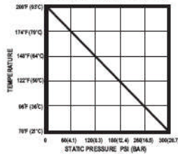
Maximum Temperature vs. Pressure
